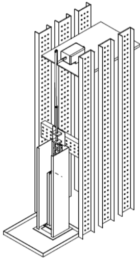
Figure 13: Layout of vertical test rig
