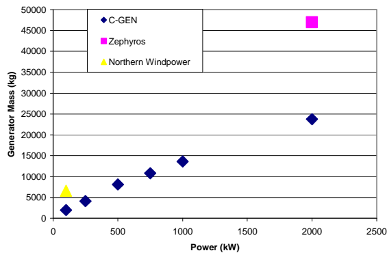
Figure 16: Scaling of C-GEN compared to conventional generators
