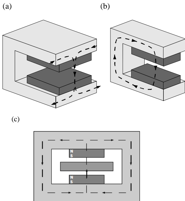
Figure 1: C-GEN magnetic flux paths, module to module flux path (a), module back flux path (b) and linear generator back flux path (c)
