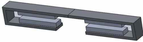
Figure 10: Core of a double sided C-GEN machine
