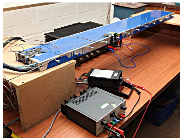
Figure 12: Submersible coil block on thermal test
