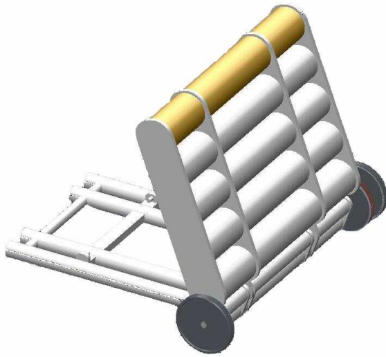
Figure 15: Possible application of rotary generators to Aquamarine Power Oyster device
